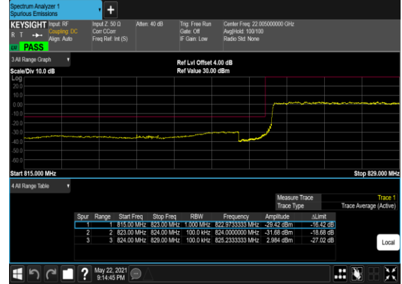
B7_N5(10M)_DFT-s-OFDM_QPSK_Outer_Full_Low_CH
