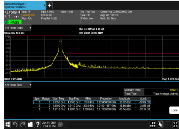
N2(20M)_DFT-s- OFDM_BPSK_Edge_1RB_Right_High_CH
