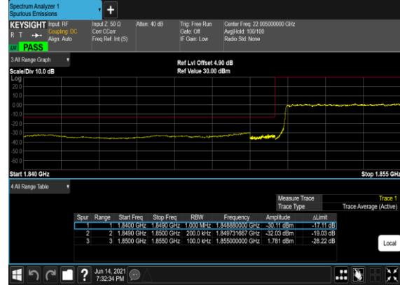
N2(20M)_DFT-s- OFDM_BPSK_Outer_Full_Low_CH
