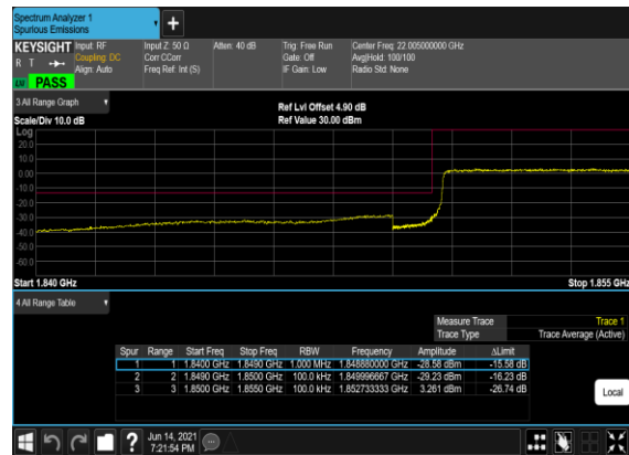
N2(10M)_DFT-s- OFDM_BPSK_Outer_Full_Low_CH
