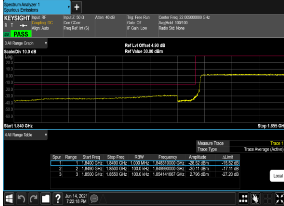
N2(10M)_DFT-s- OFDM_QPSK_Outer_Full_Low_CH
