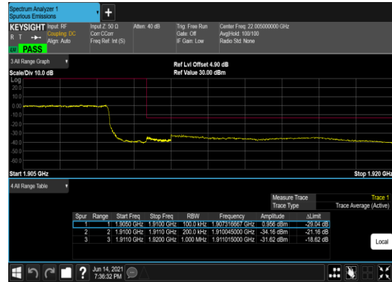
N2(20M)_DFT-s- OFDM_BPSK_Outer_Full_High_CH
