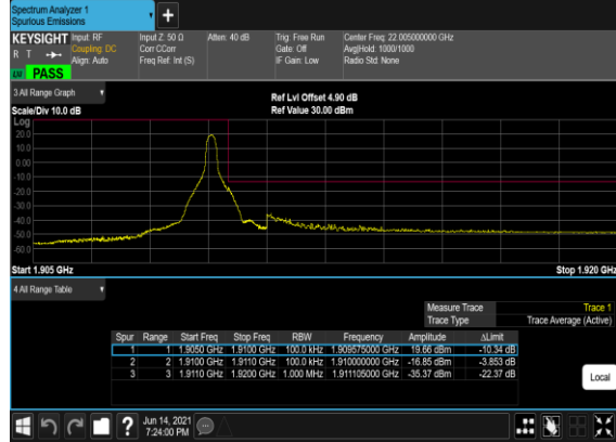
N2(10M)_DFT-s- OFDM_BPSK_Edge_1RB_Right_High_CH
