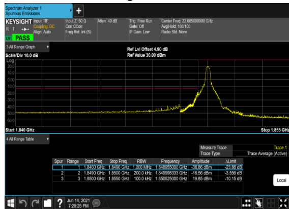
N2(20M)_DFT-s- OFDM_BPSK_Edge_1RB_Left_Low_CH
