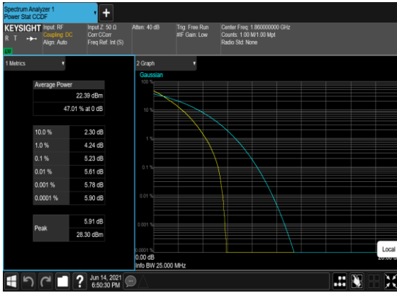
N2(20M)_DFT-s-OFDM_QPSK_Outer_Full_Low_CH
