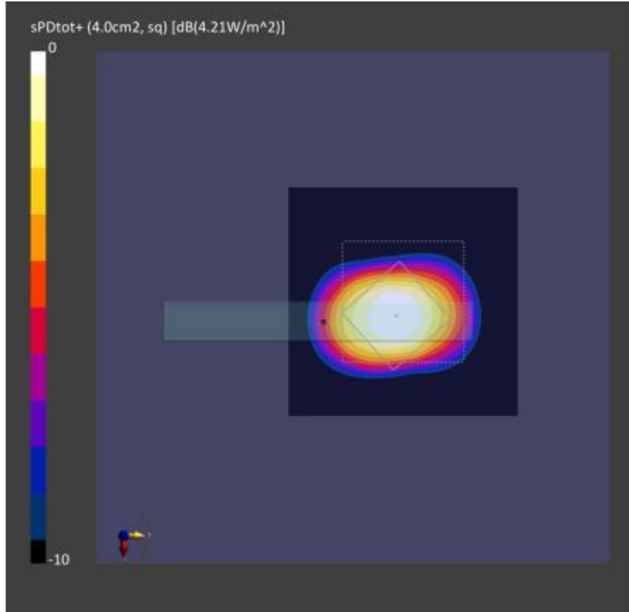
Figure 8-3: 4cm2-averaged power density distribution measured at input.power.limit of 4.21 dBm on the Right Side surface for n260 beam 15
