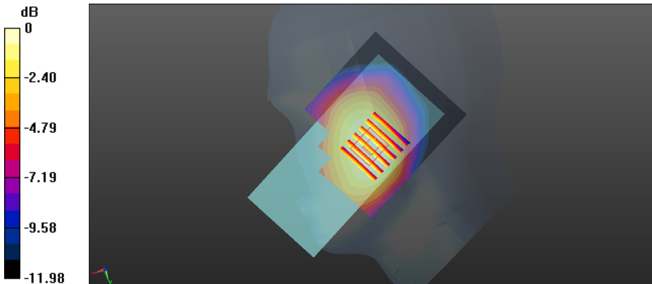
0 dB = 0.402 W/kg
