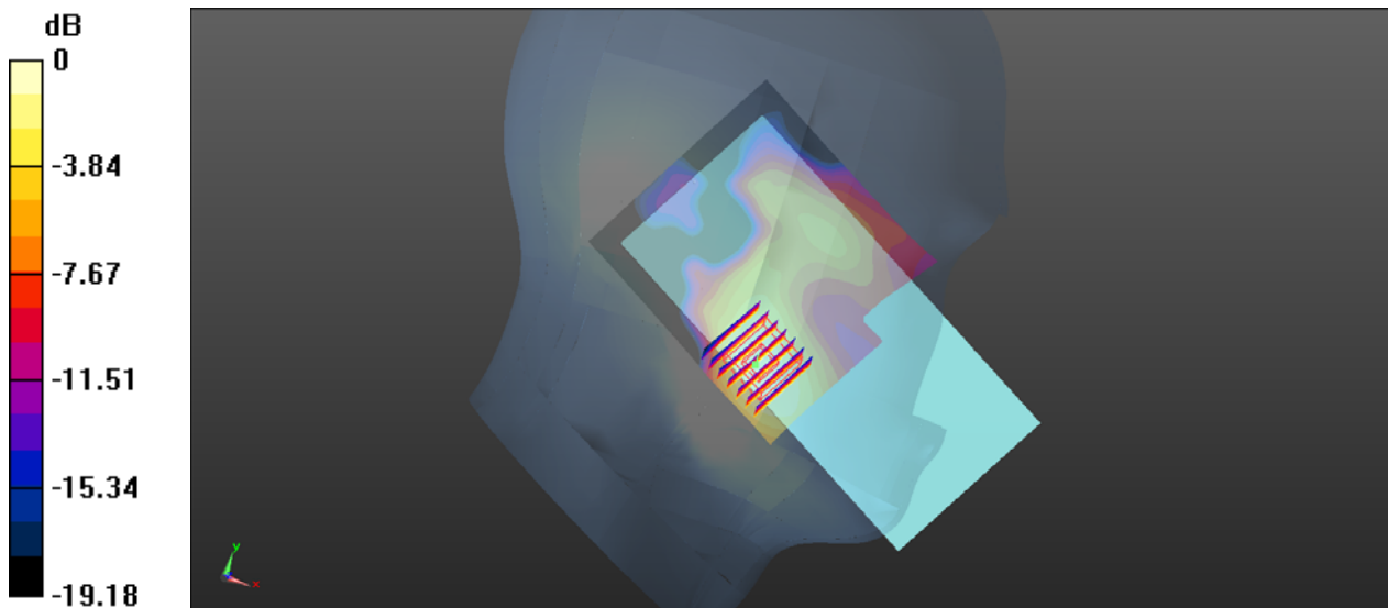
0 dB = 0.217 W/kg
