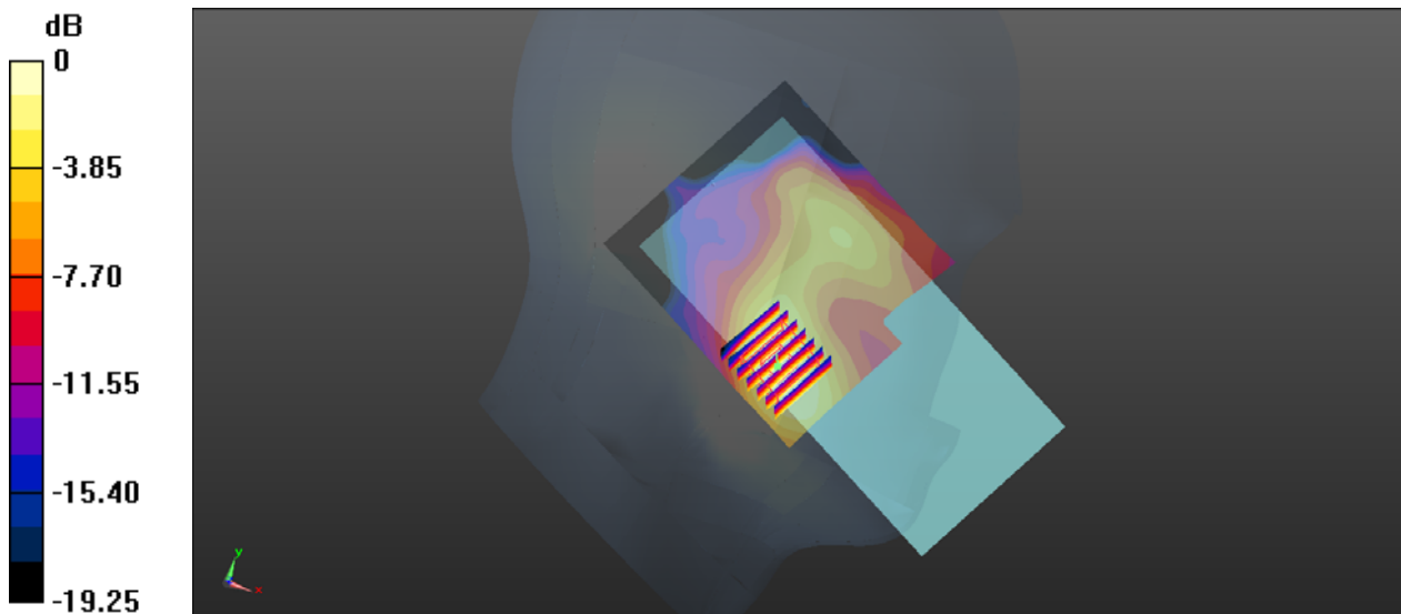
0 dB = 0.256 W/kg
