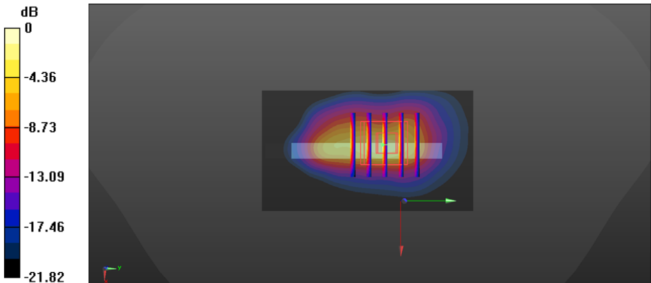
0 dB = 13.6 W/kg
