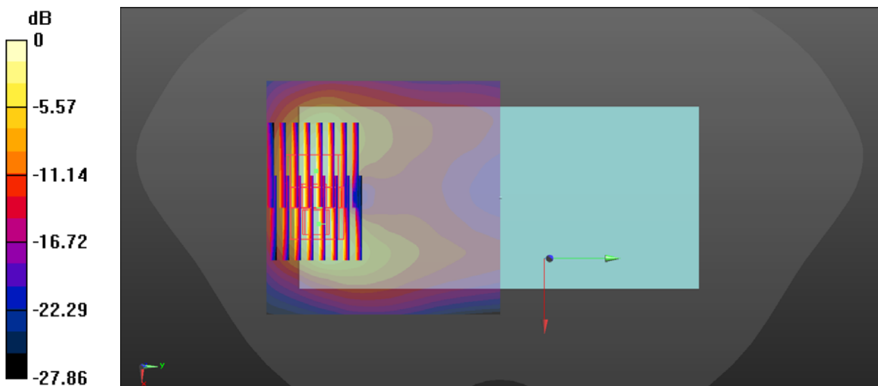
0 dB = 1.68 W/kg
