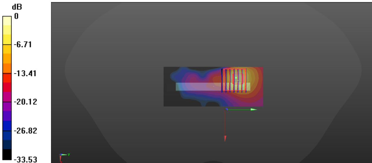
0 dB = 7.32 W/kg
