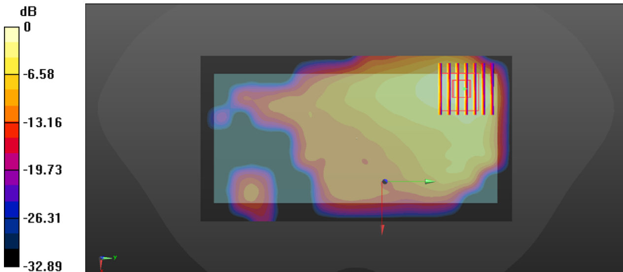
0 dB = 0.153 W/kg
