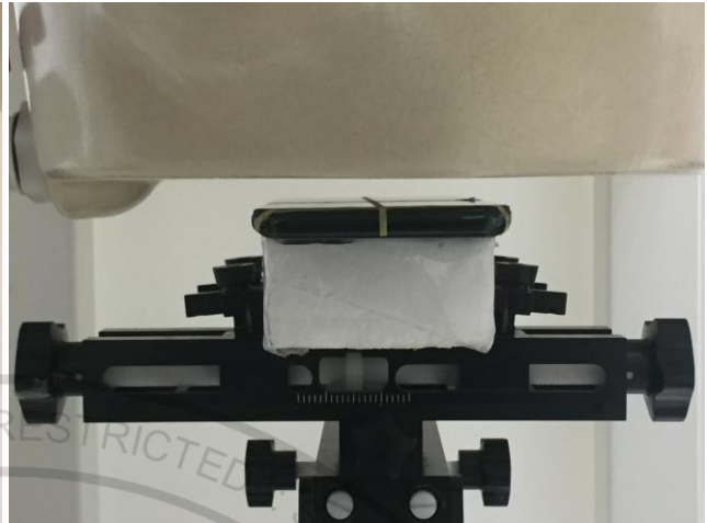
Front, Test Separation 9 mm
