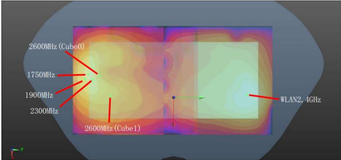
WWAN+WLAN2.4GHz_0mm
