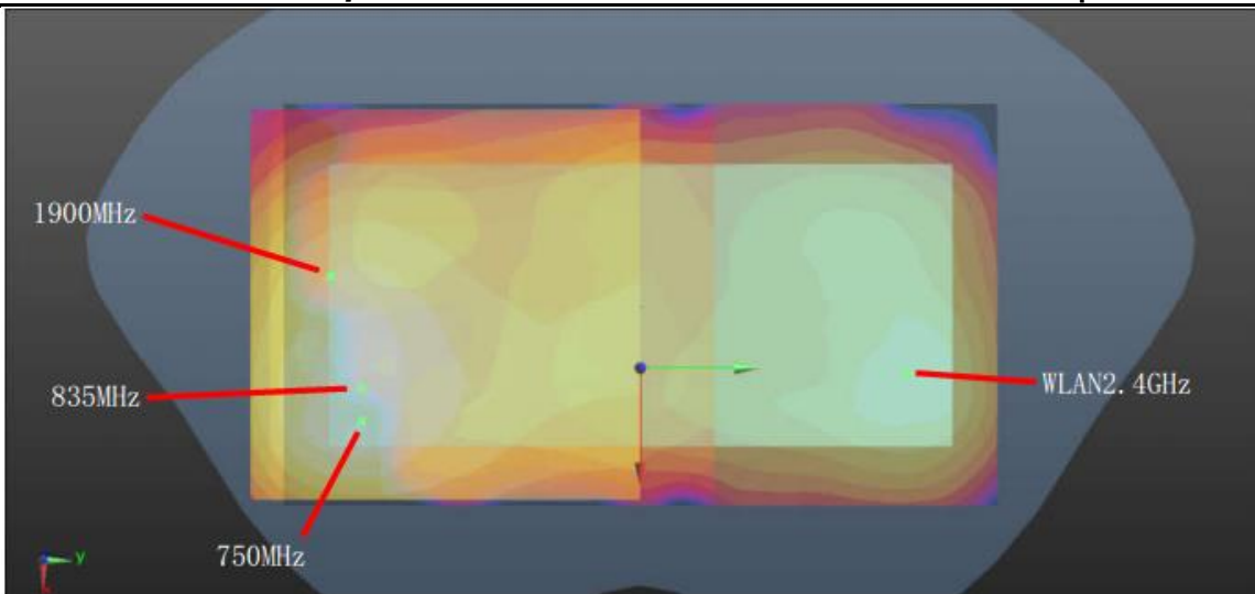
WWAN+WLAN2.4GHz_5mm
