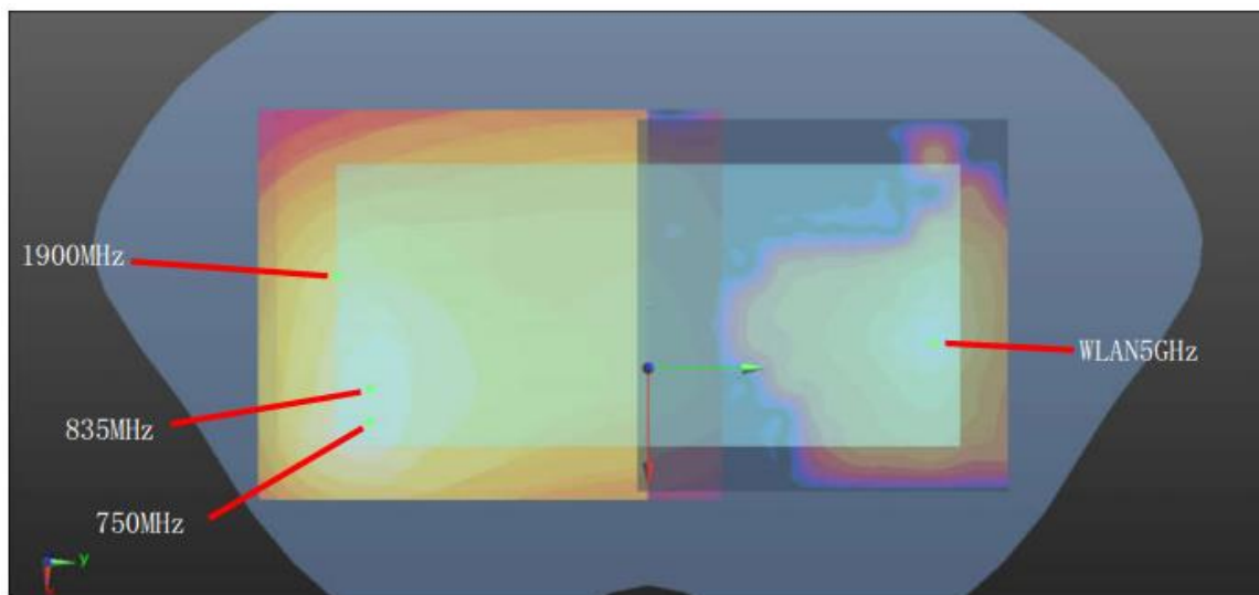
WWAN+WLAN5GHz_5mm
