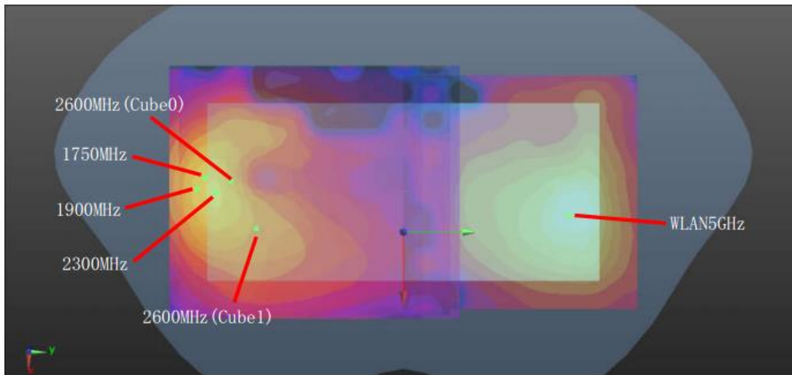
WWAN+WLAN5GHz_0mm
