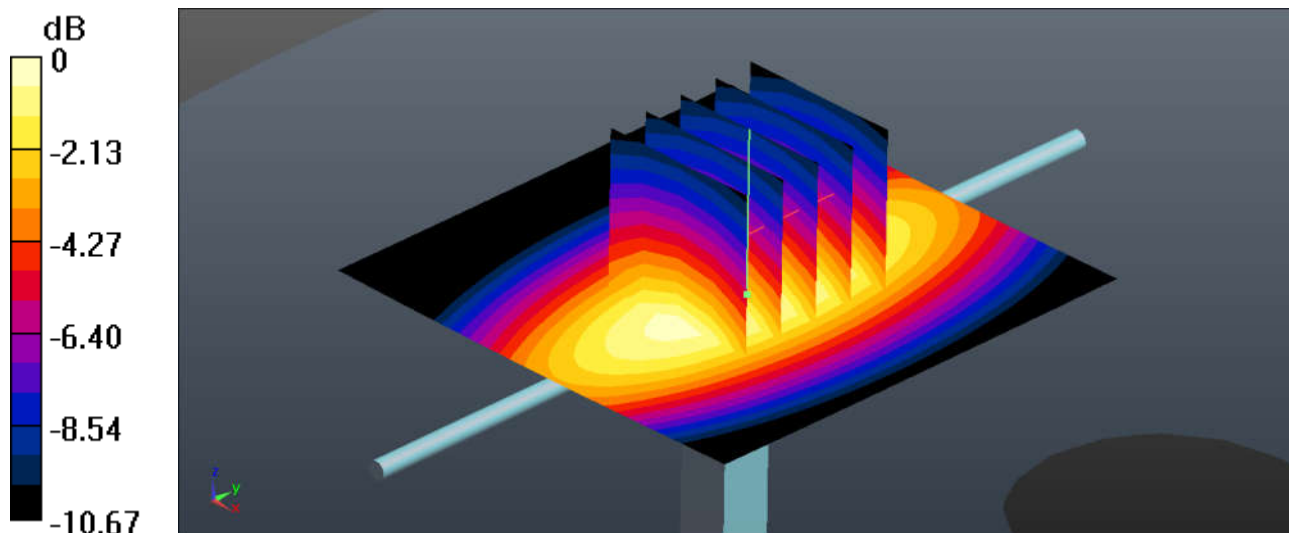
0 dB = 3.31 W/kg
