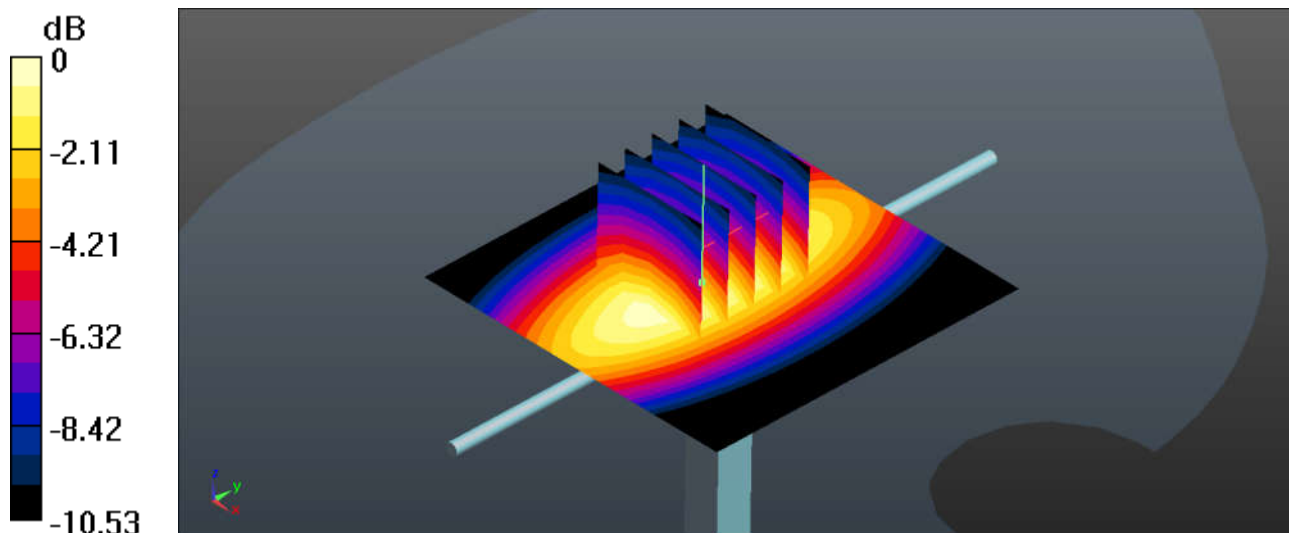
0 dB = 3.08 W/kg
