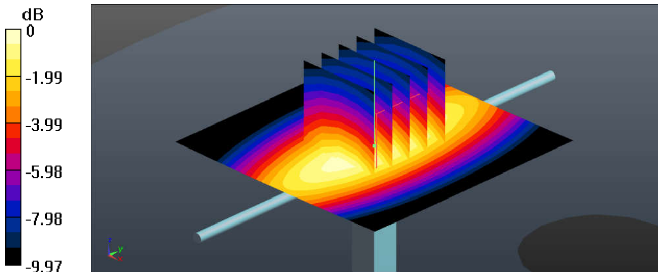
0 dB = 2.78 W/kg
