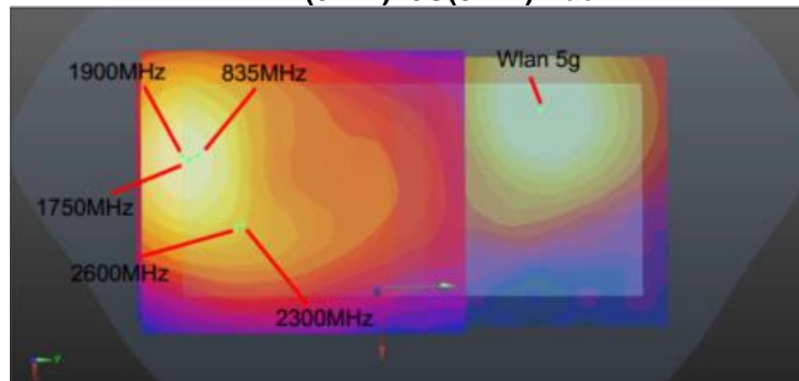
WWAN(19mm)+5G(19mm) Back
