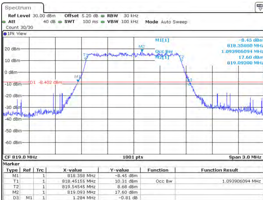
Band26-1.4MHz-QPSK-26740-6RB#0-1.094
