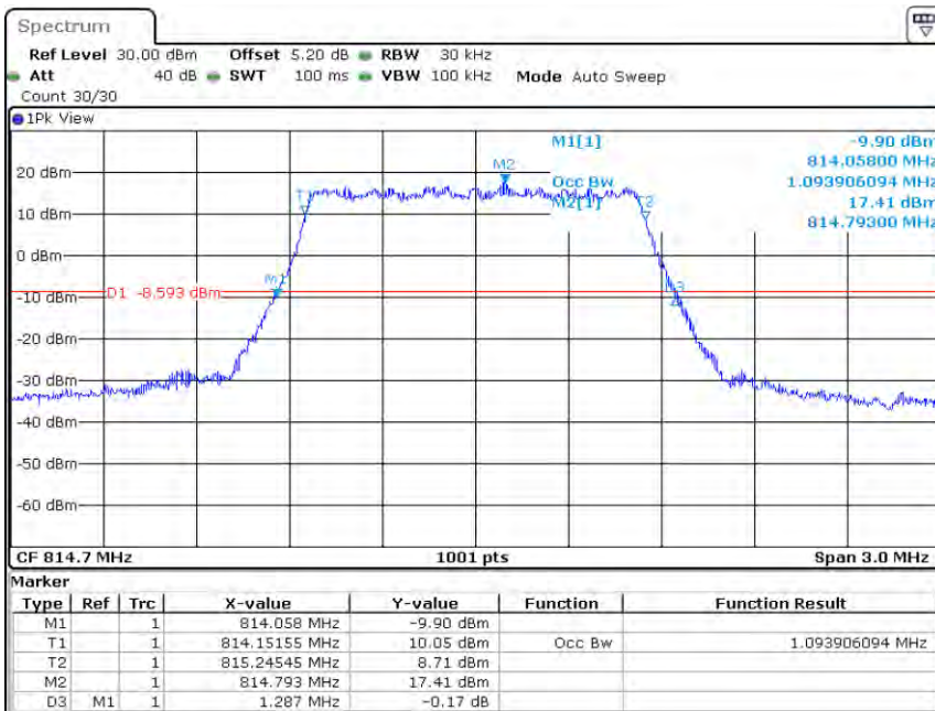
Band26-1.4MHz-QPSK-26697-6RB#0-1.094
