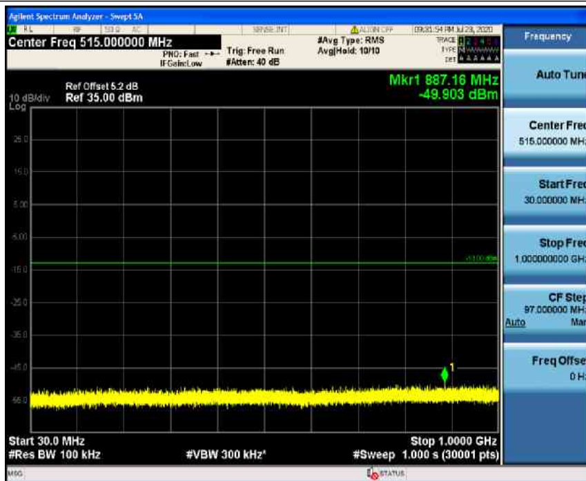
Band2-20MHz-64QAM-18900-1RB#0-Range1:30~1000MHz
