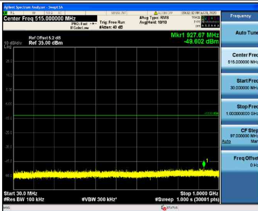
Band2-20MHz-64QAM-19100-1RB#0-Range1:30~1000MHz
