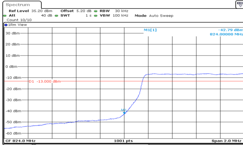
Band5-1.4MHz-64QAM-20407-6RB#0
