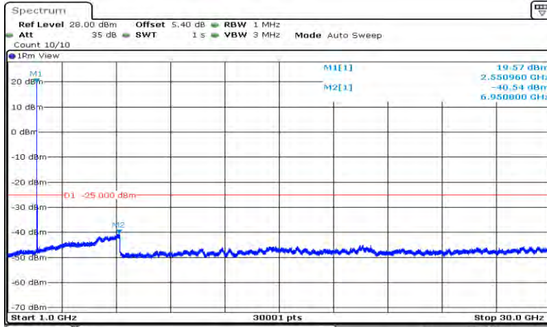
Band7-20MHz-64QAM-21350-1RB#0-Range2:1000~30000MHz
