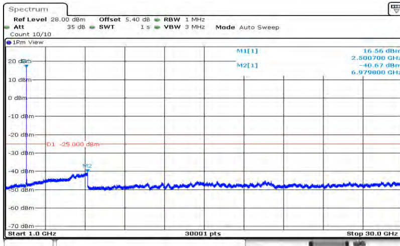
Band7-20MHz-64QAM-20850-1RB#0-Range2:1000~30000MHz
