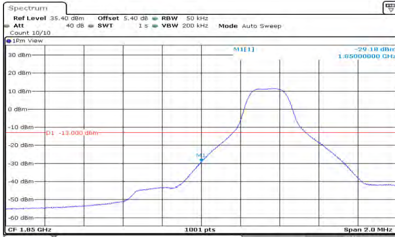
Band2-5MHz-64QAM-18625-25RB#0
