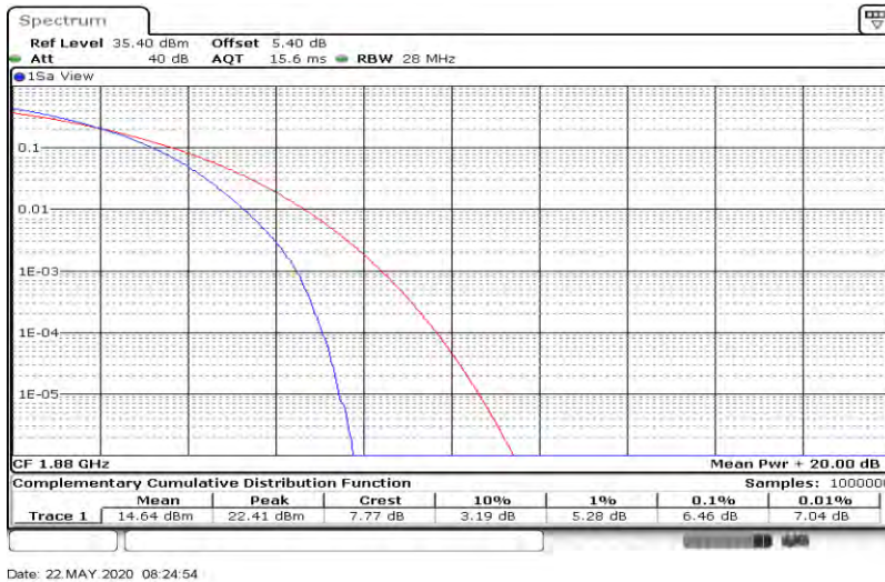
Band2-20MHz-64QAM-19100-100RB#0
