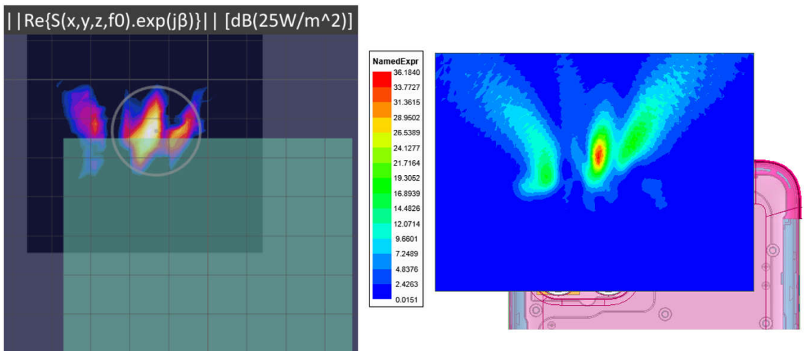
Figure 2.3.7.1-22 Measured (left) and Simulated (right) peak power density distributions for the worst case found in the Top surface measurement plane for n260 ( Top module, beam 153, back surface )
