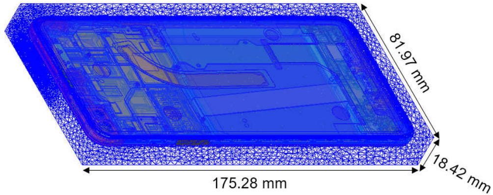
Figure 2.3.3-1: The HFSS mesh in a model of the device. After finding the simulated electric and magnetic ( \vec{E} and \vec{H} ) fields, the Poynting vector is calculated based on “peak” (i.e. non-RMS) field values in a grid with a 1 mm step, on the appropriate measurement planes as defined in previous sections. The Poynting vector at each spatial point is readily available in HFSS through the “Field Calculator” navigation option. The magnitude of the real part of the Poynting vector (all X, Y, Z components) at each spatial point i.e. the point power density is exported from HFSS to do the averaging. The spatially averaged power density at each point on a given surface is then calculated by taking the average of the point power density over a 4 square cm area. Thus the total power density (all X, Y, Z components) through any given surface is used to calculate the averaged power density.
