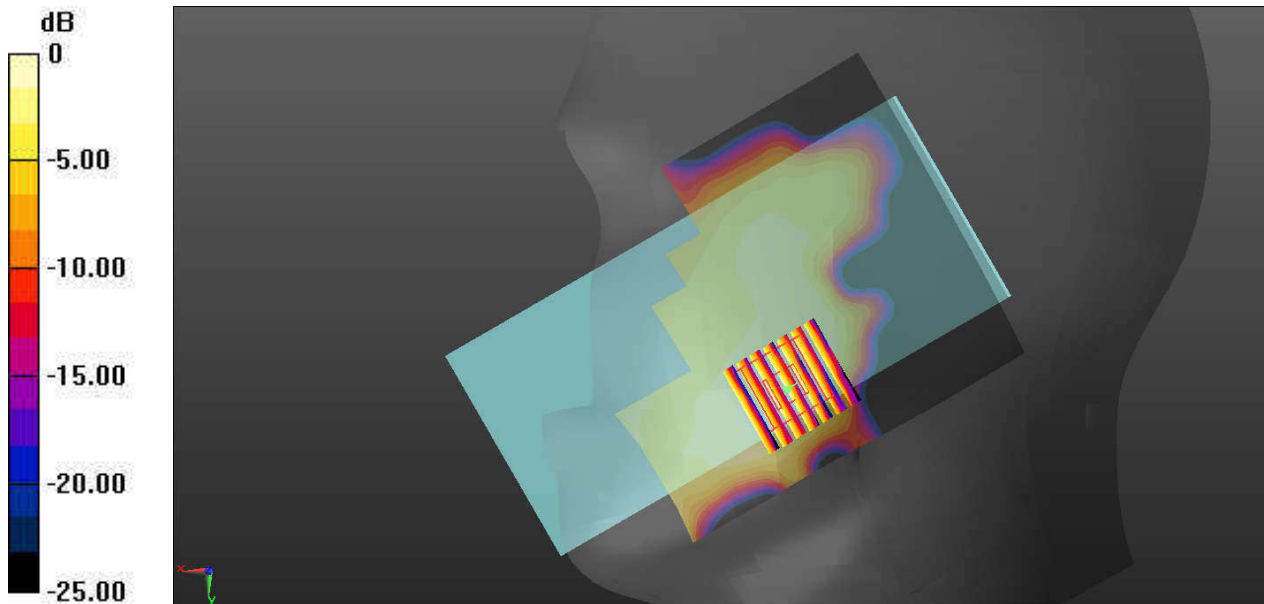
0 dB = 0.0685 W/kg = -11.64 dBW/kg
