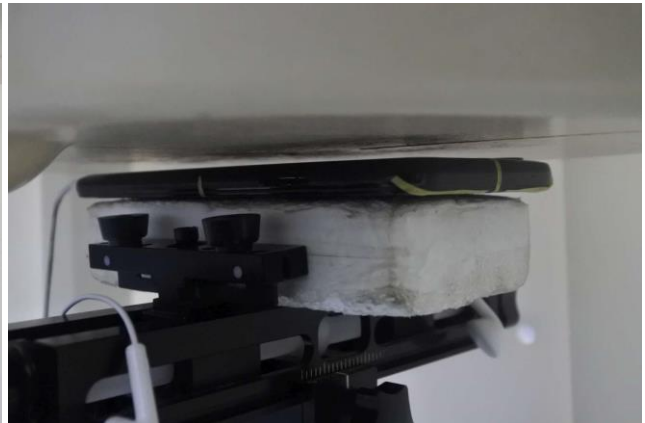
Back with handset, Test Separation 5 mm
