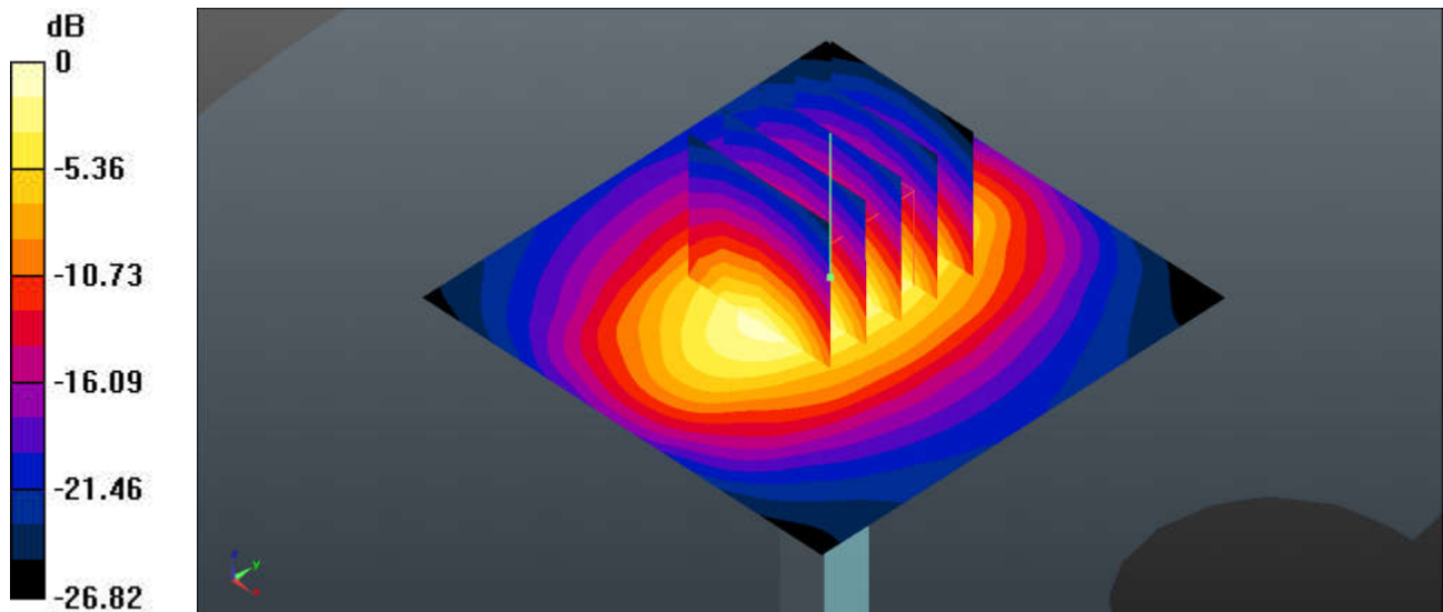
0 dB = 12.7 W/kg = 11.04 dBW/kg
