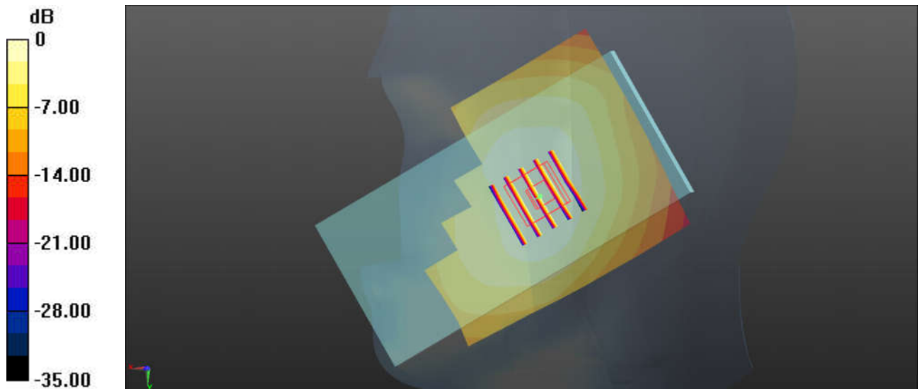
0 dB = 0.422 W/kg = -3.75 dBW/kg
