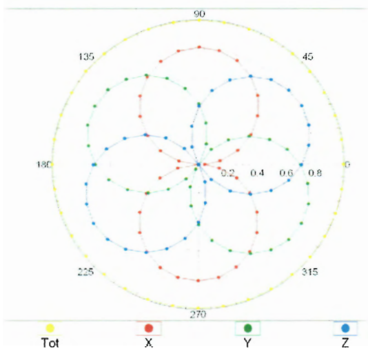
f=600 MHz,TEM
