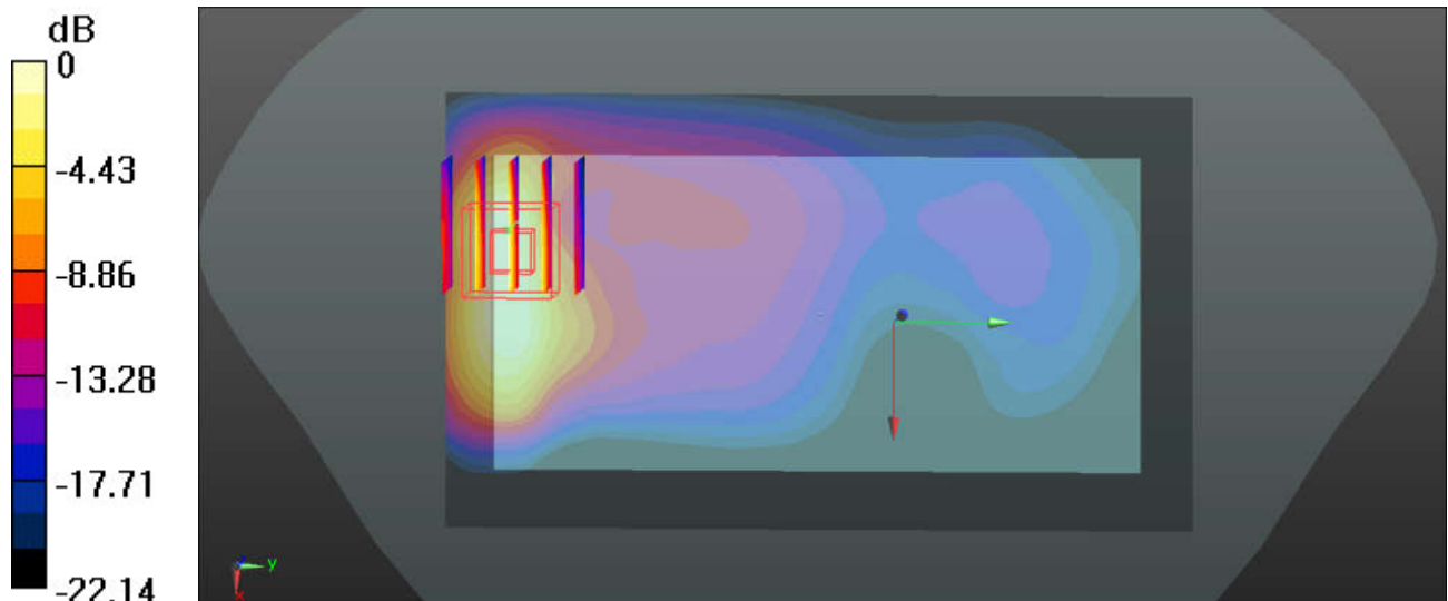
0 dB = 1.34 W/kg
