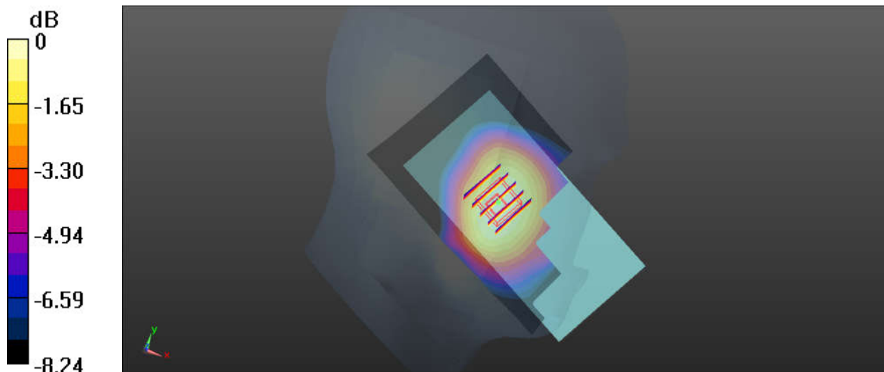
0 dB = 0.229 W/kg
