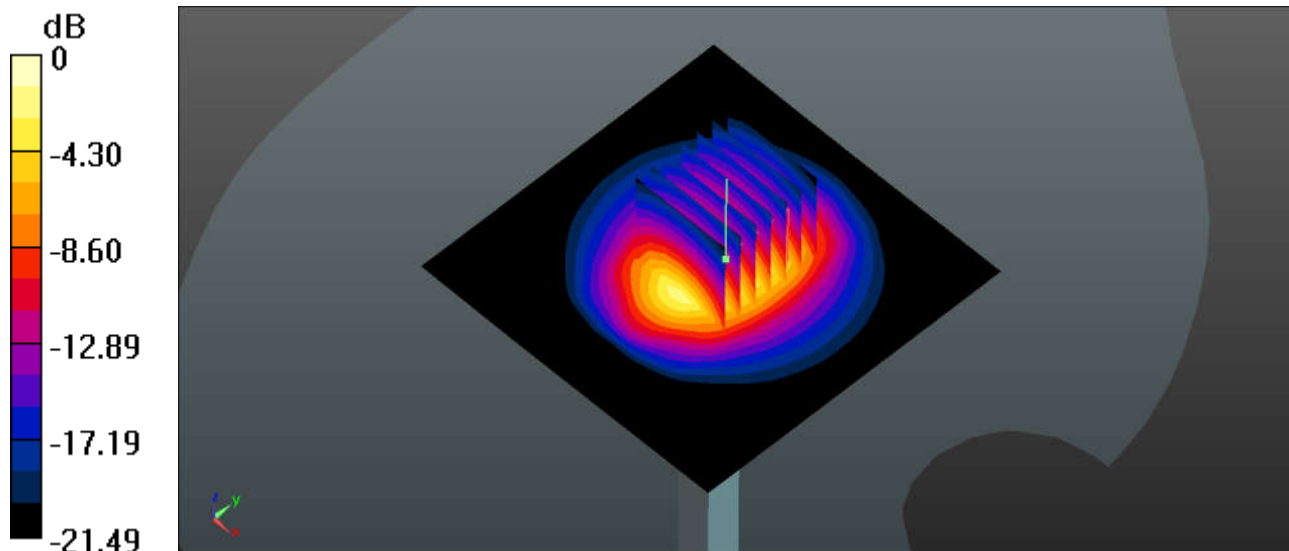
0 dB = 19.4 W/kg
