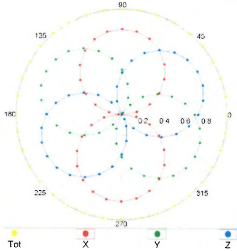
f=600 MHz,TEM
