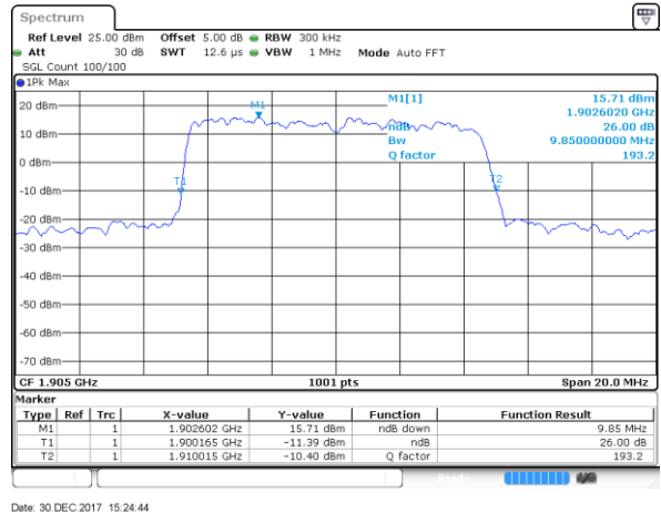
Highest Channel / 10MHz / 64QAM
