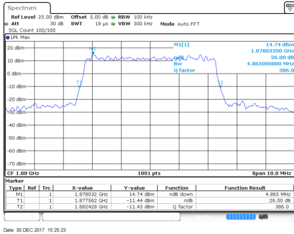
Highest Channel / 5MHz / 64QAM
