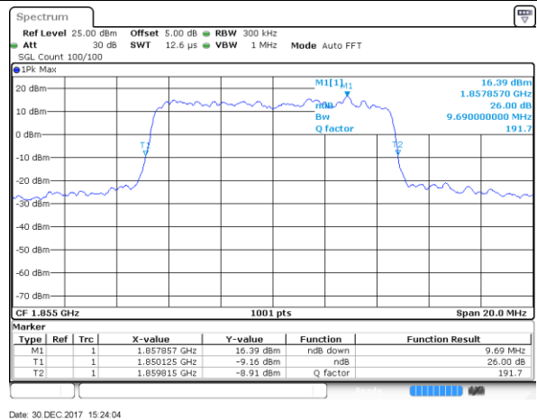
Middle Channel / 10MHz / 64QAM
