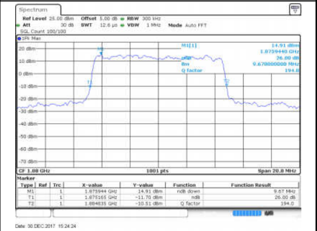
Highest Channel / 10MHz / 64QAM
