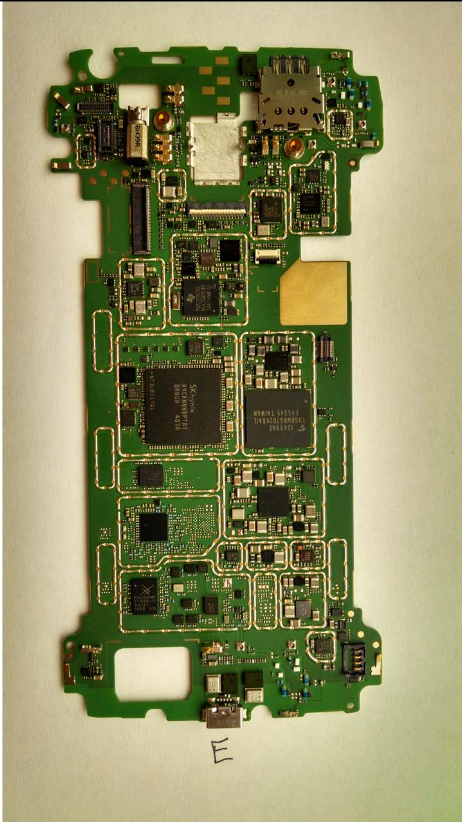
Photograph 9-2: Front side view of the device's PC Board, Shields Removed.
