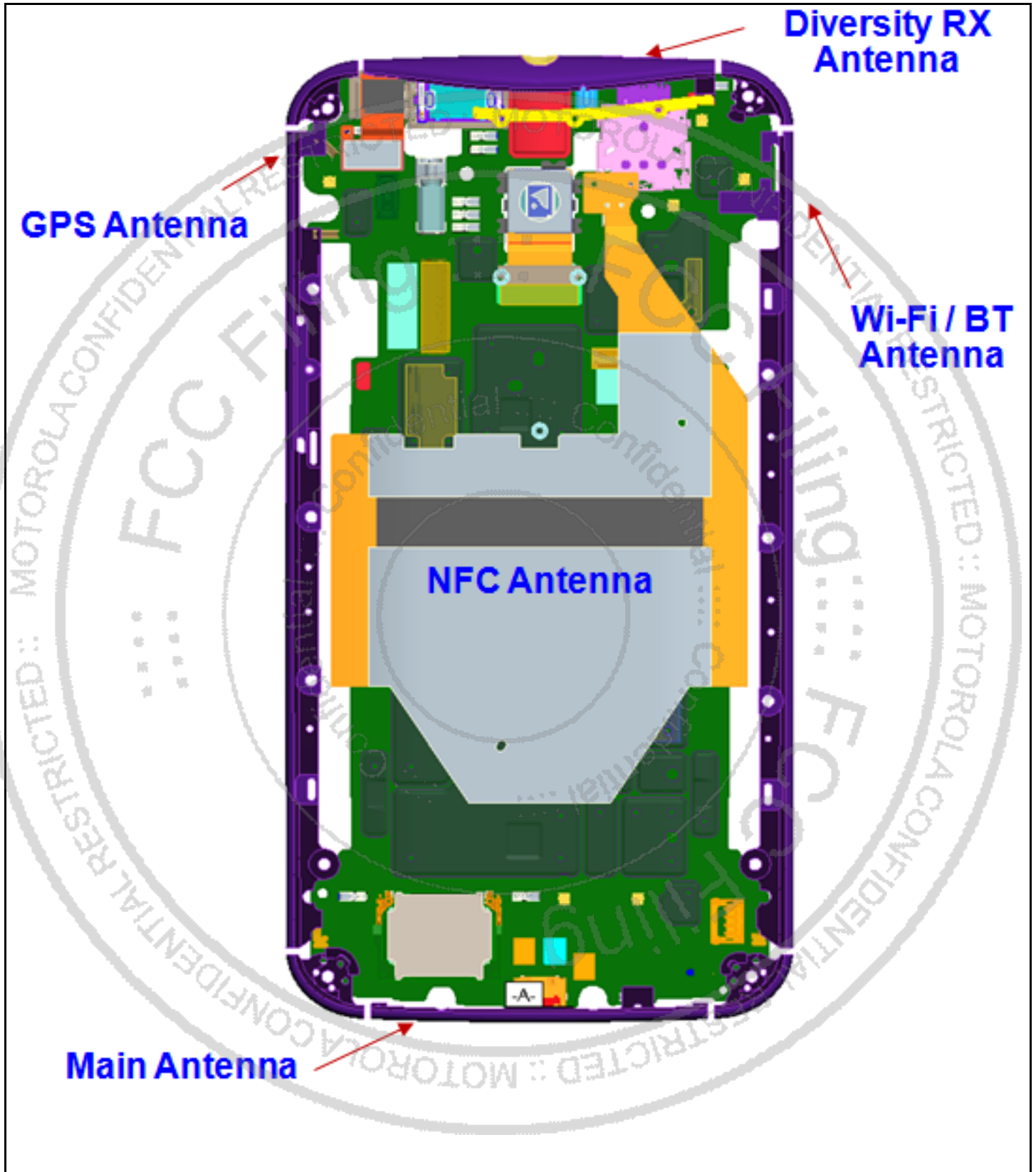
Photograph 9-4: Antenna Locations.
