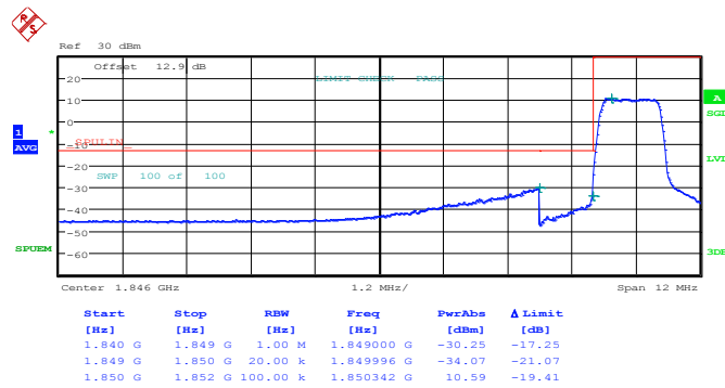
Lower Band Edge Plot for QPSK-RB Size 6, RB Offset 0
