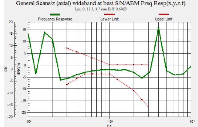
Fig 7.2 GSM1900 Ch661
