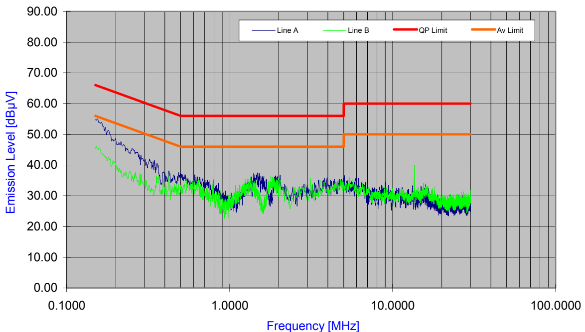
Plot 6-35. Line Conducted Plot with 802.11b
