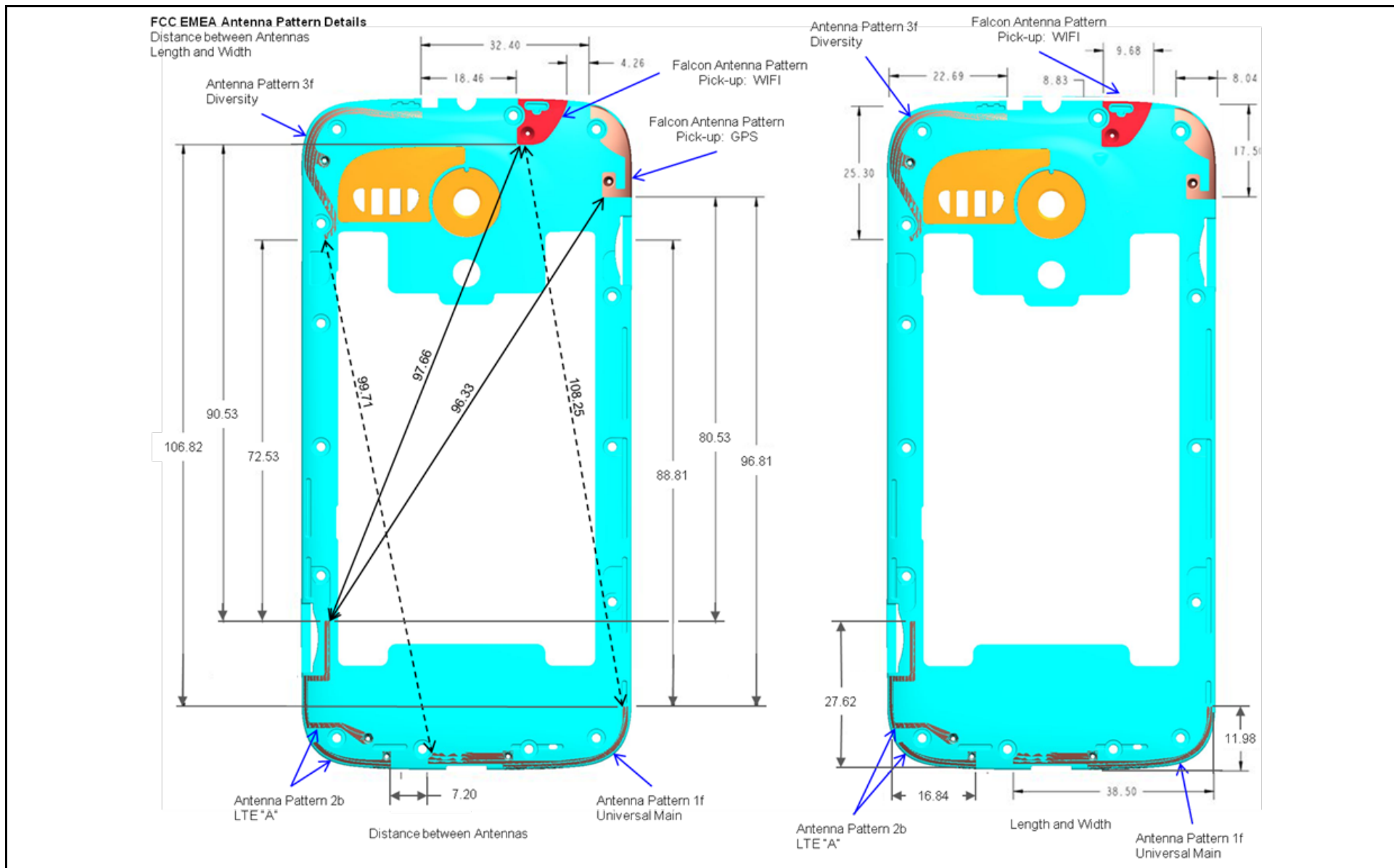
Photograph 9-5: Antenna Spacings.
