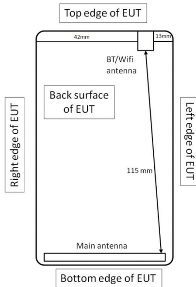
Figure 2: Antenna Separation Distances
