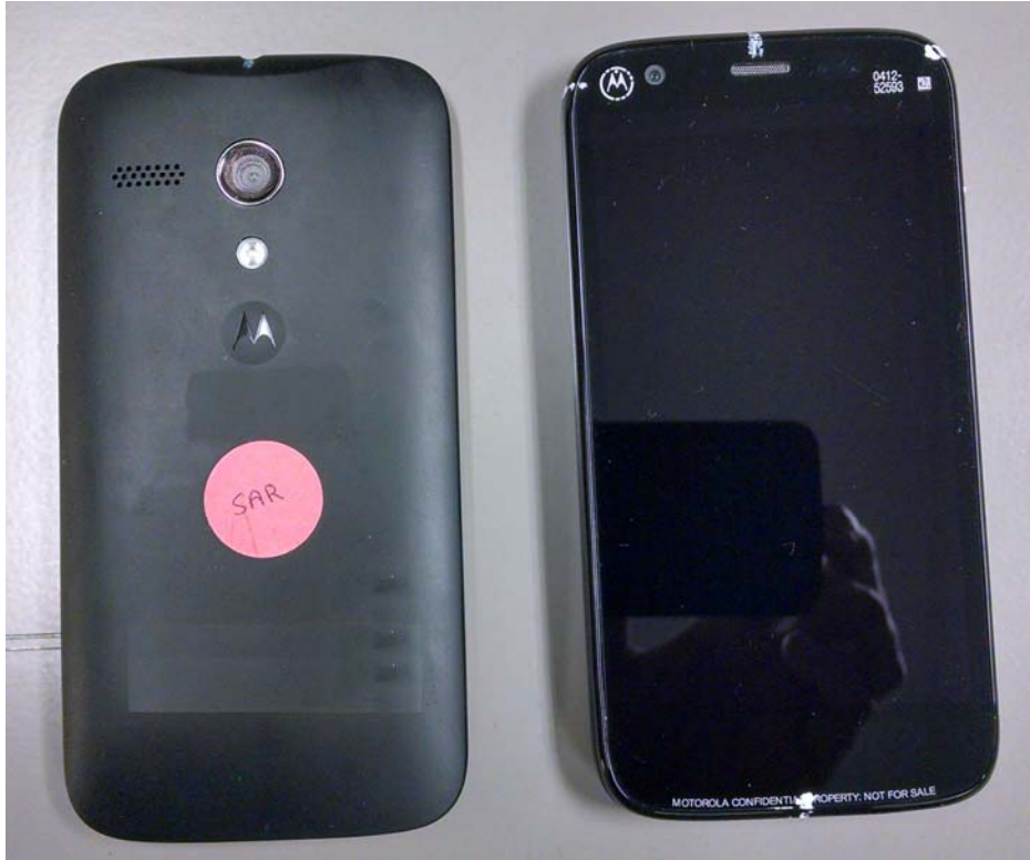
Figure 1: Phone Front and Back
