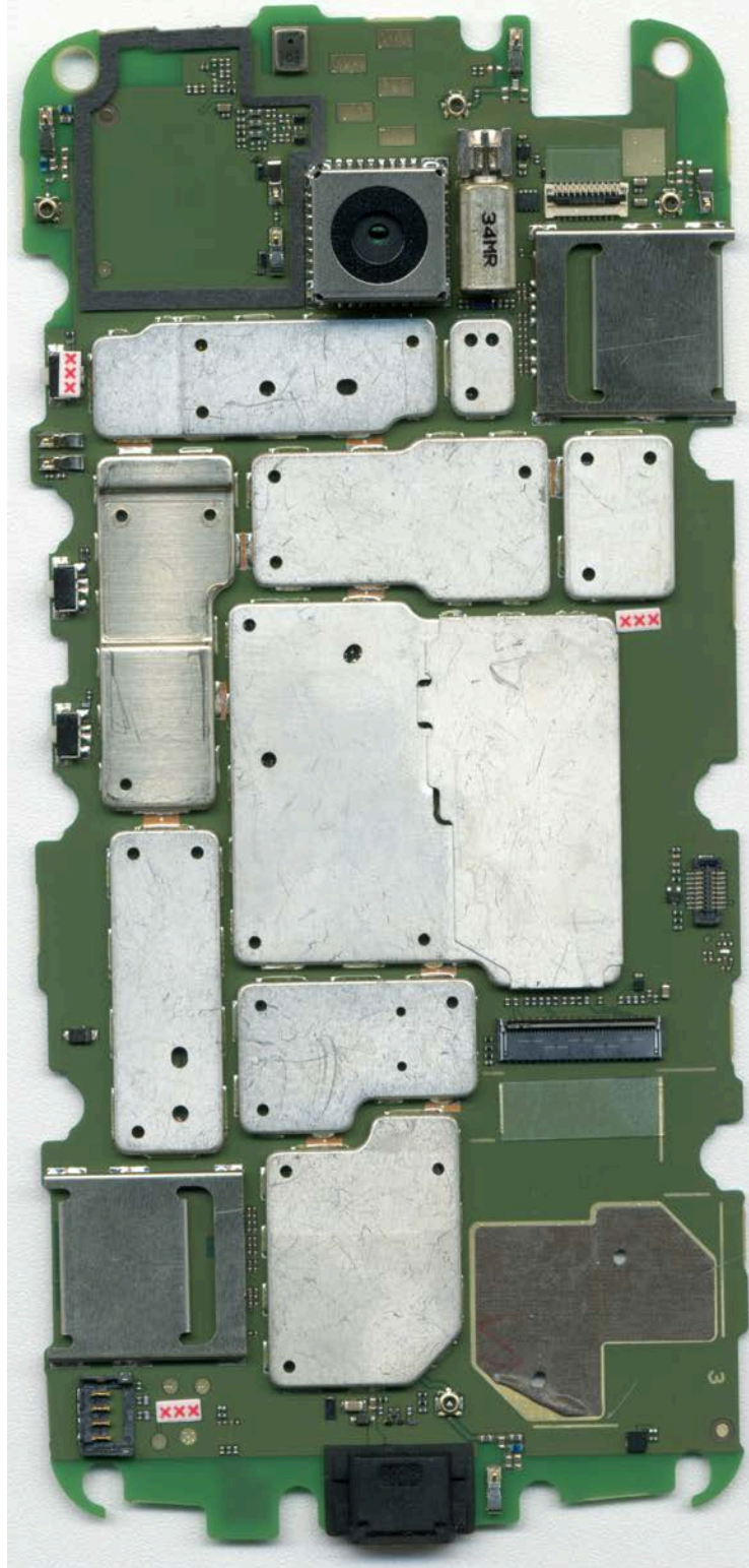
Photograph 9-1: Component side view of the device's PC Board, Shields in place.
