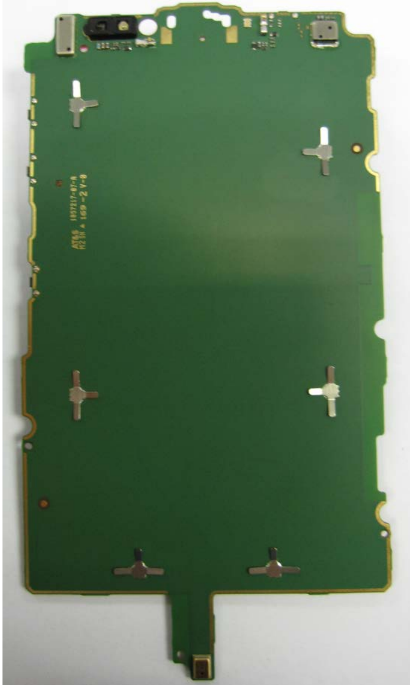
Photograph 9-1: Front side view of the device's Personality PC Board, Shields in place.
