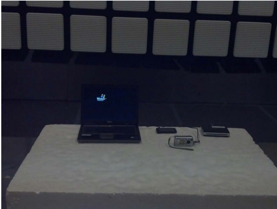
Radiated Emissions – Computer Peripheral
