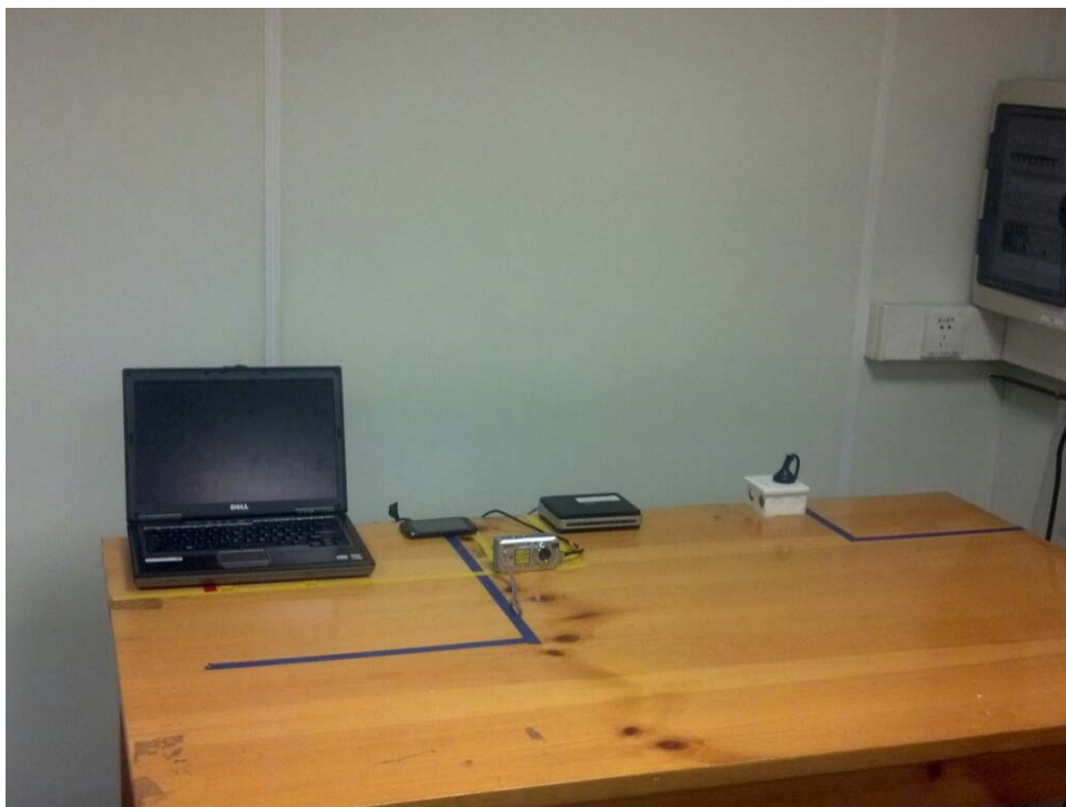
AC Line Conducted Emissions – Computer Peripheral
