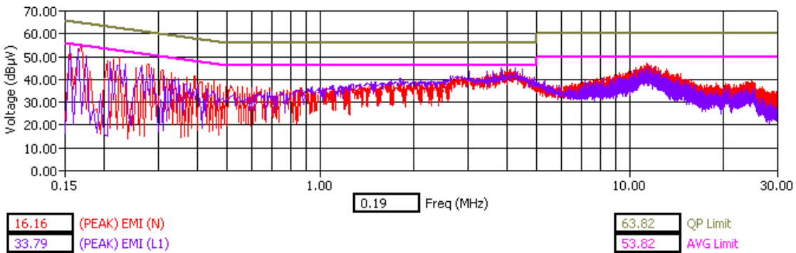
Bluetooth – Hopping - Tx Mode – Peak Detector
