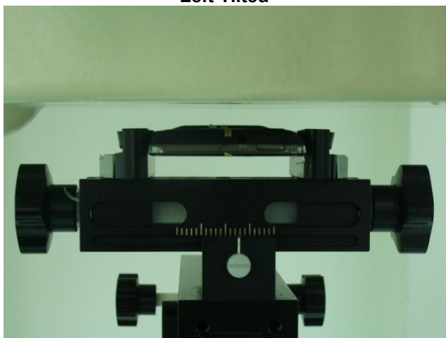
Back of the DUT with Phantom 1 cm Gap (DUT without Earphone)
