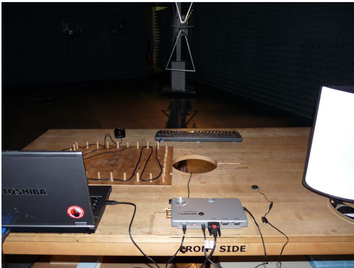
setup for the test radiated emissions
