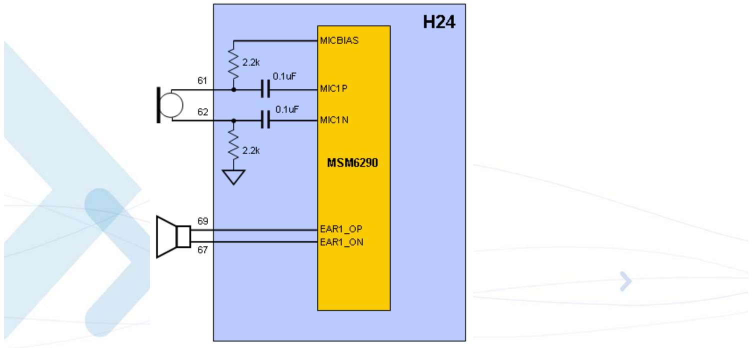
Figure 2-10: Handset Interface
