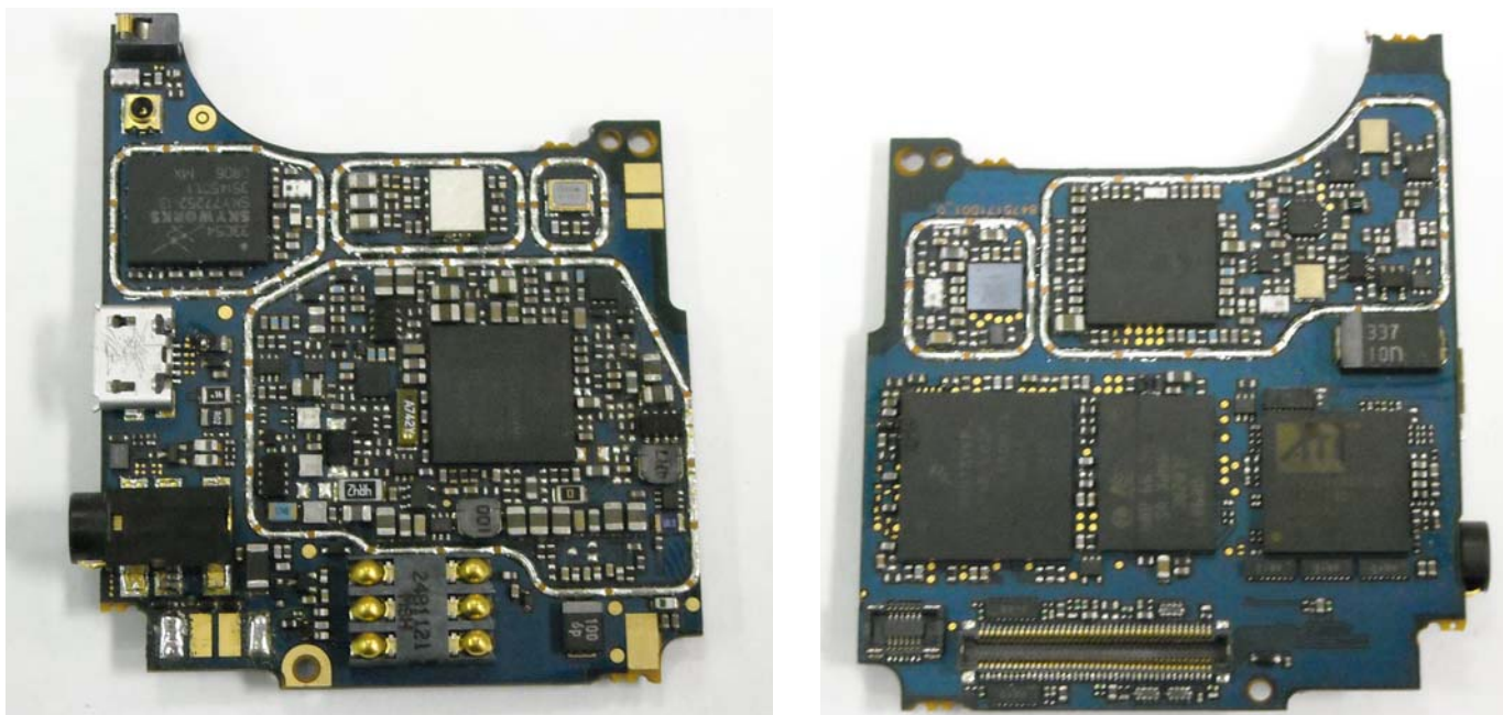
Photograph 9-3: Front and Back side view of radio PC Board, without shields.
