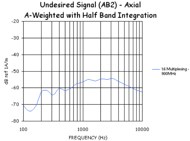
Figure 9-4-2: 900 MHz Undesired Signal (1:6).
