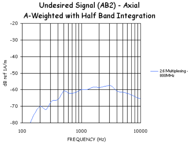
Figure 9-2-1: 800 MHz Undesired Signal (2:6).
