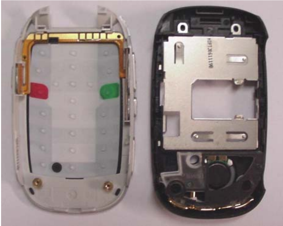
Inside Front Housing
