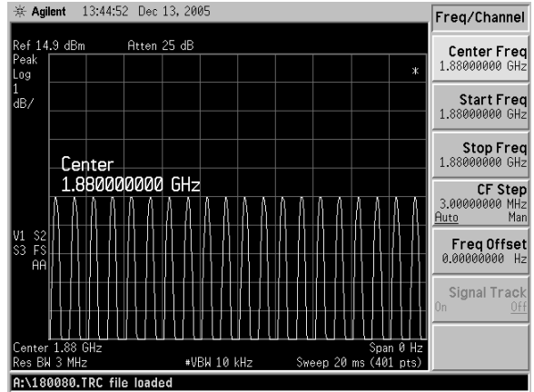
80% AM 1880 MHz
