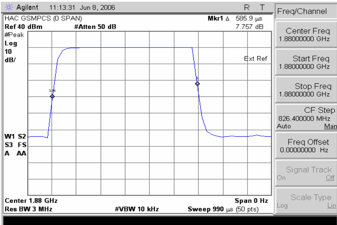
1880 MHz (0 span)
