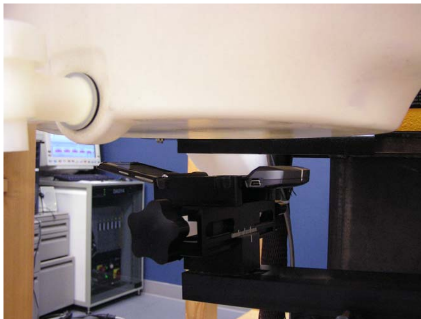
Figure 9 – Transceiver in Face Dispatch position, 25 mm from Phantom
