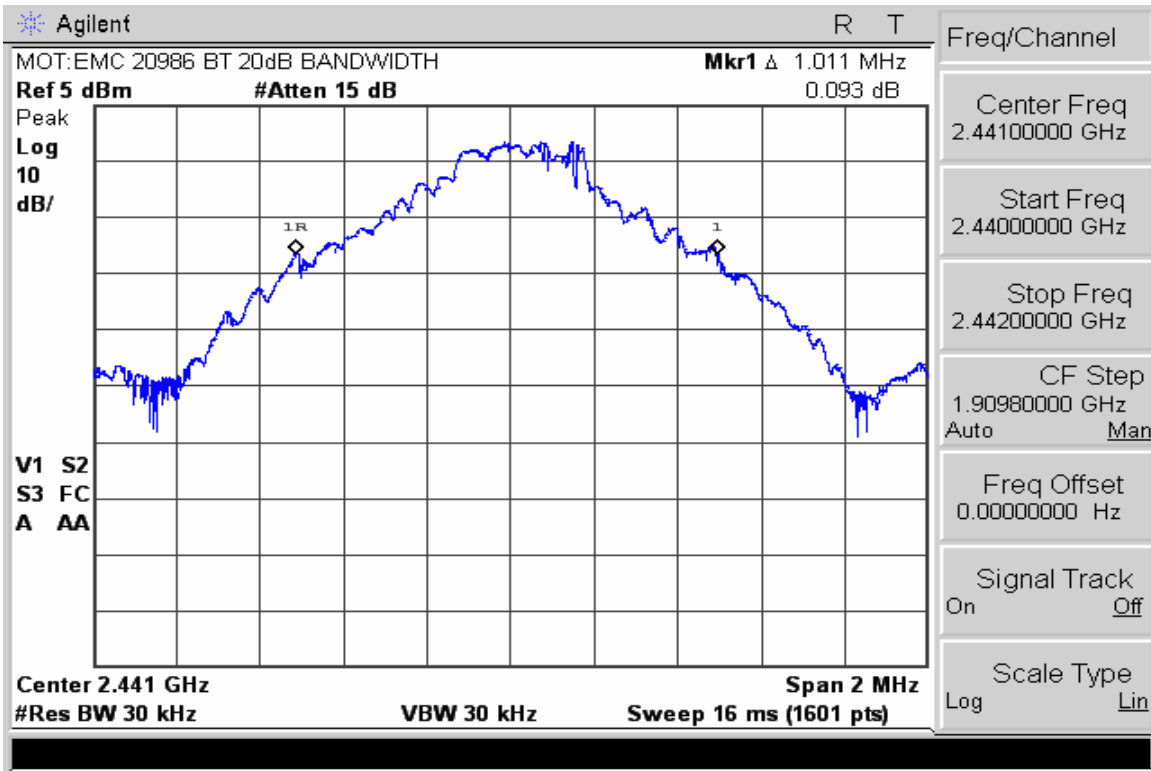
20dB Bandwidth
