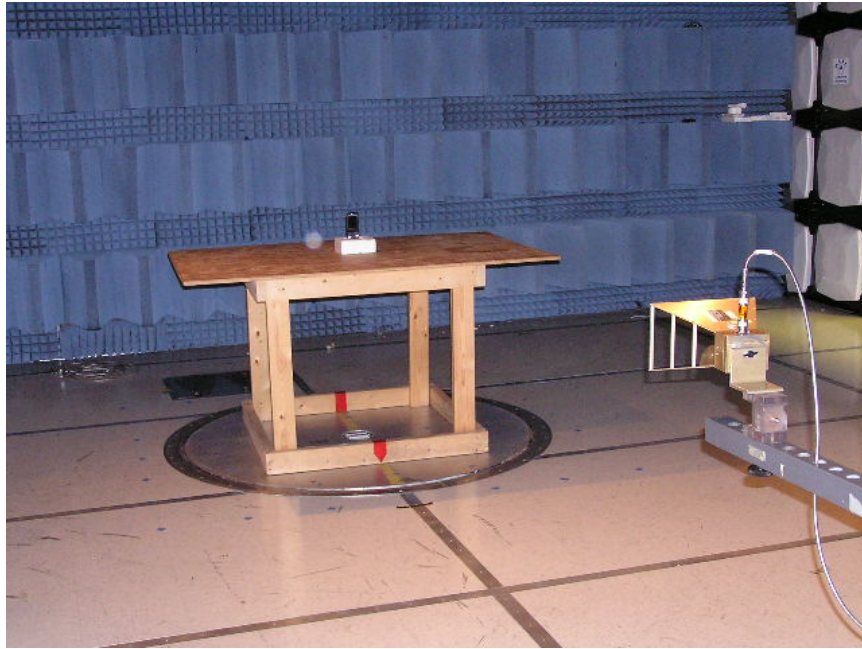
A.1 Radiated Emissions Measurement (Representative Photo- Not actual Phone tested)
