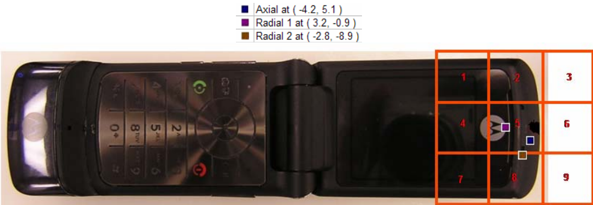
Figure A4-3. Phone Open – 5cm x 5cm grid for Near Field Measurements and T-coil Measured Point locations
