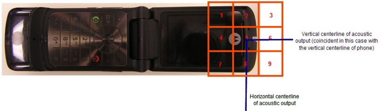
Figure A6-2. Phone Open - Orientation of Wireless Device and Measurement Plane
