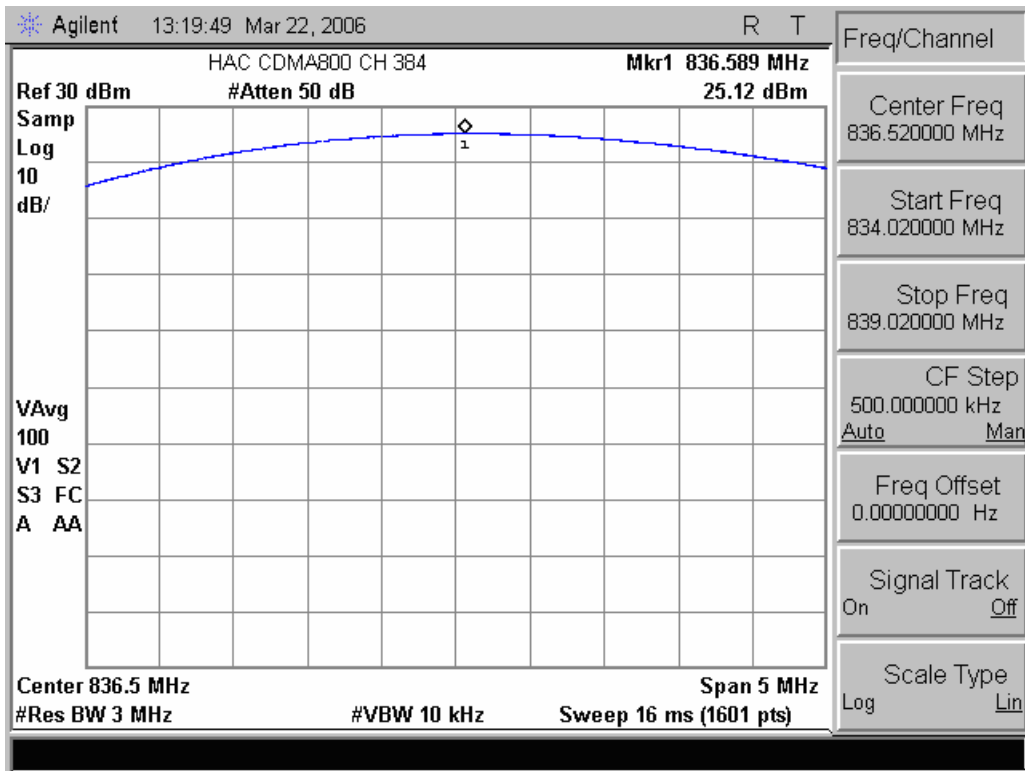
836.5 MHz (wideband)
