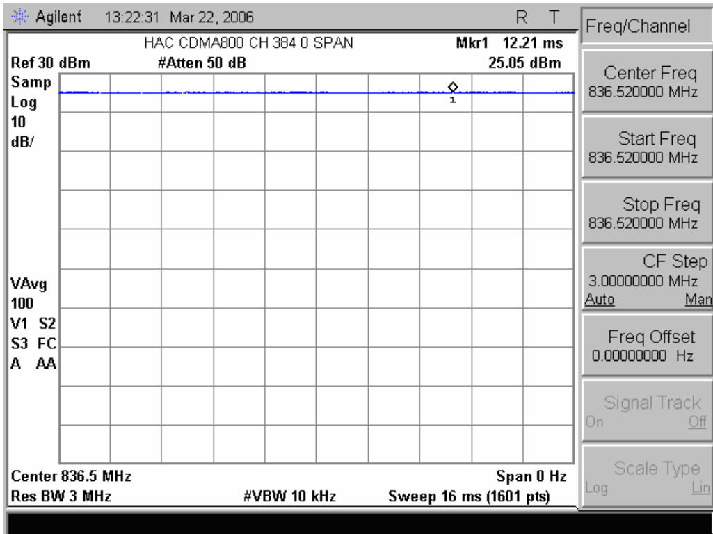
836.5 MHz (0 span)
