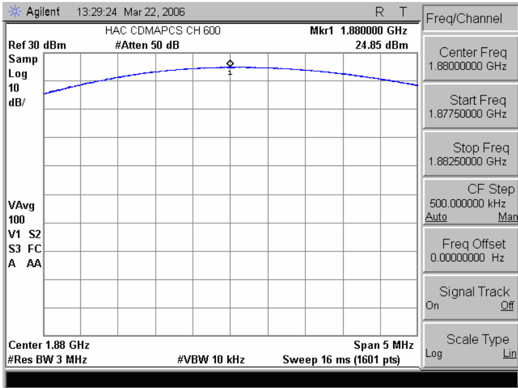
1880.0 MHz (wideband)
