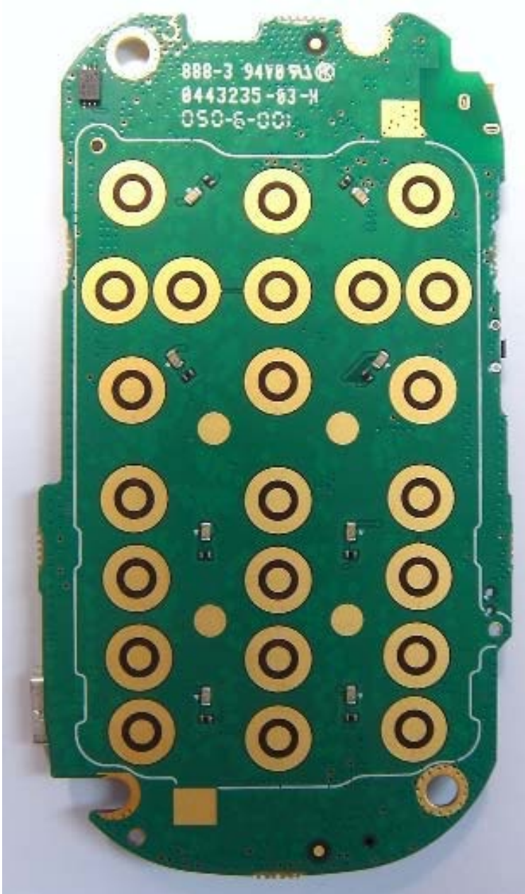
Front View (Keypad PCB Layout)
