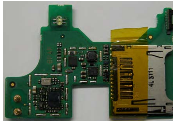
Daughter Board without shields
