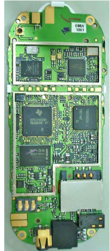
Main Board Bottom w/out shields
